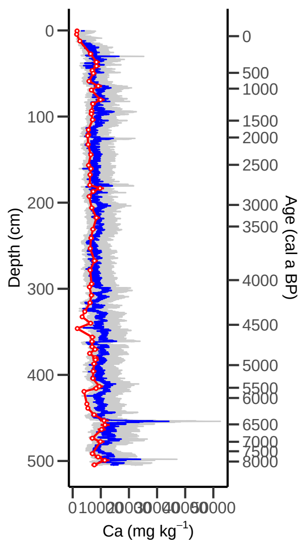
BI10: PLSR Ca Predictions with
