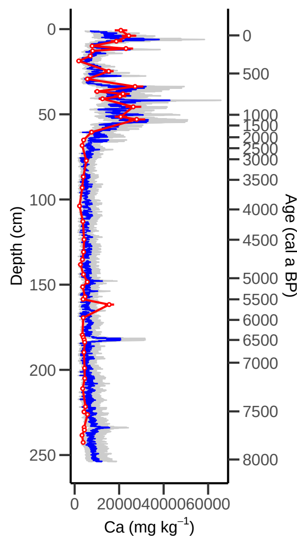
KER1: PLSR Ca Predictions with
