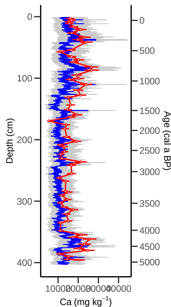
HER42PB: PLSR Ca Prediction
