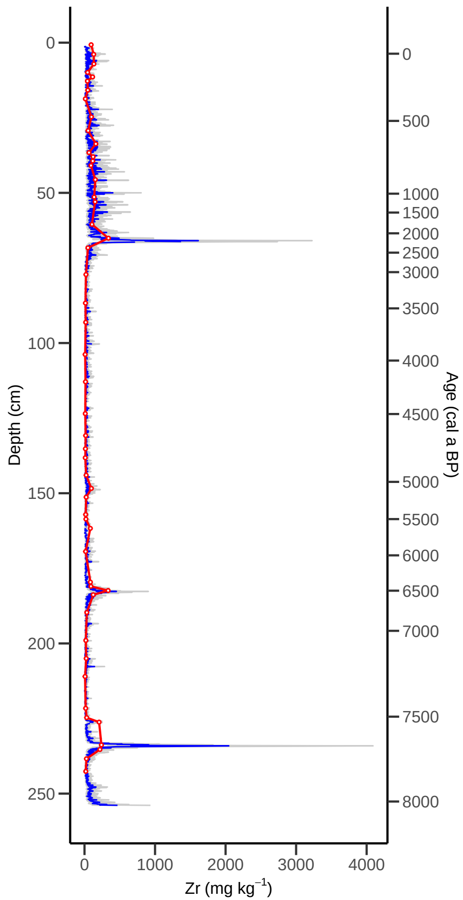
KER1: PLSR Zr Predictions with Confidence Intervals
