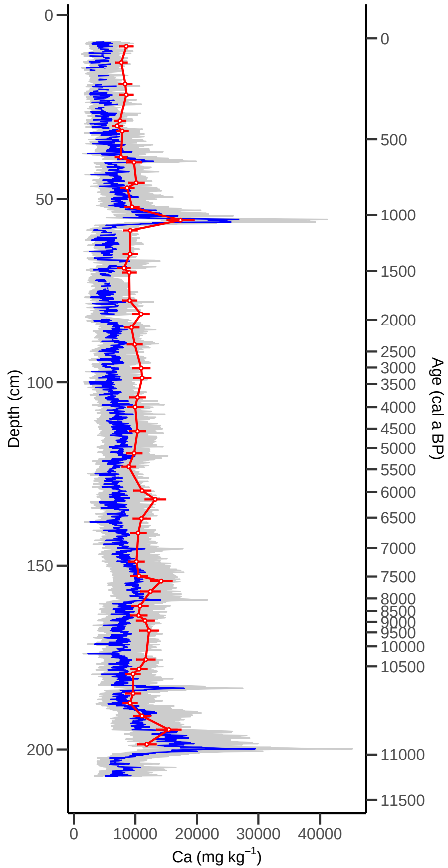
KER3: PLSR Ca Predictions with Confidence Interv
