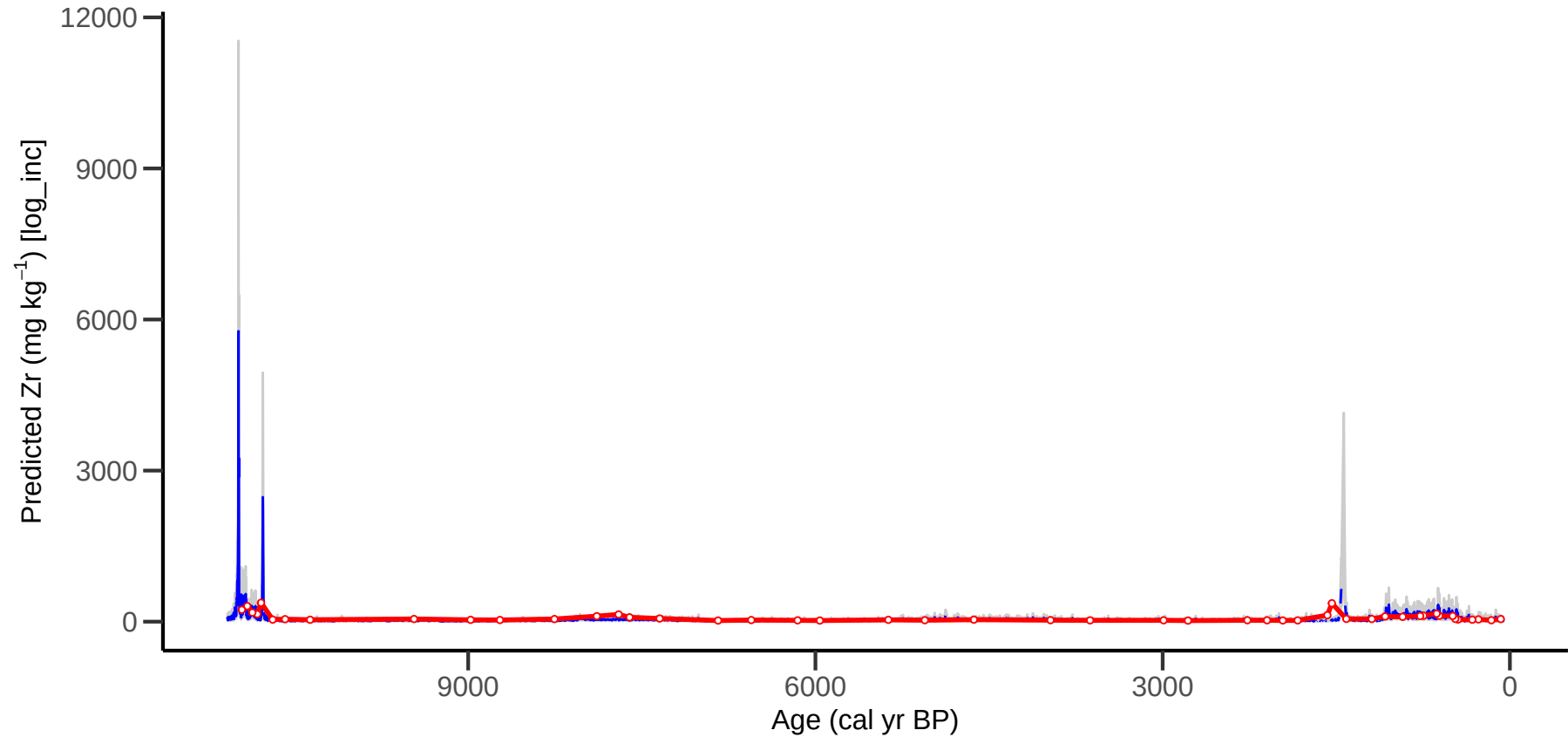
KER3: PLSR Zr Predictions with Confidence Interval (log_inc model)
