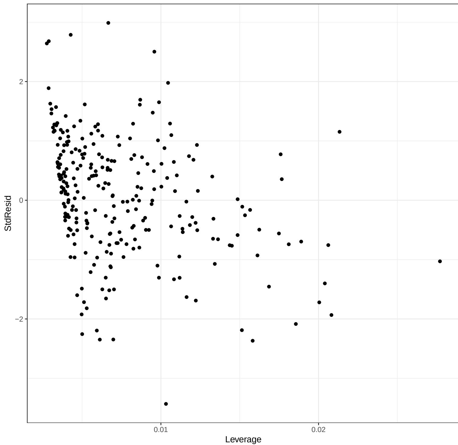
Fe OLS_weighted – Leverage Plot
