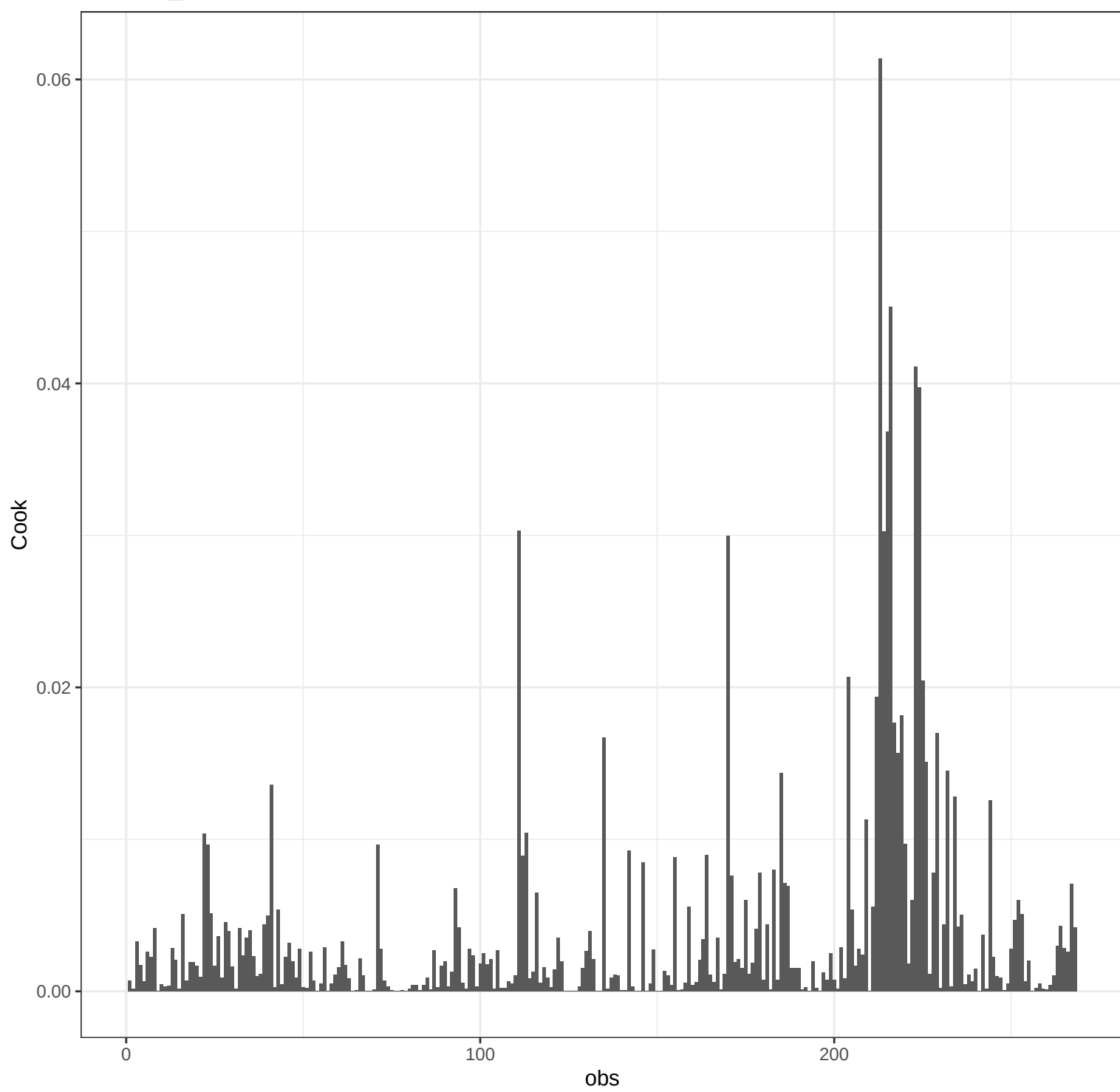
Fe OLS_weighted – Cook's Distance
