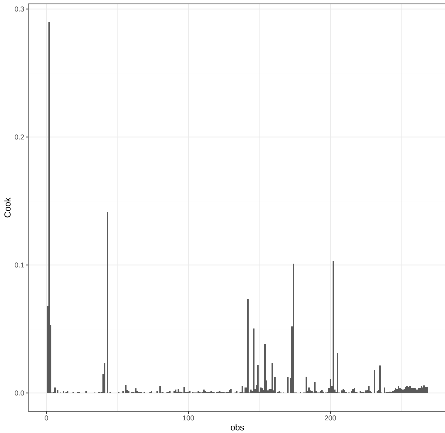
Sr OLS_weighted – Cook's Distance
