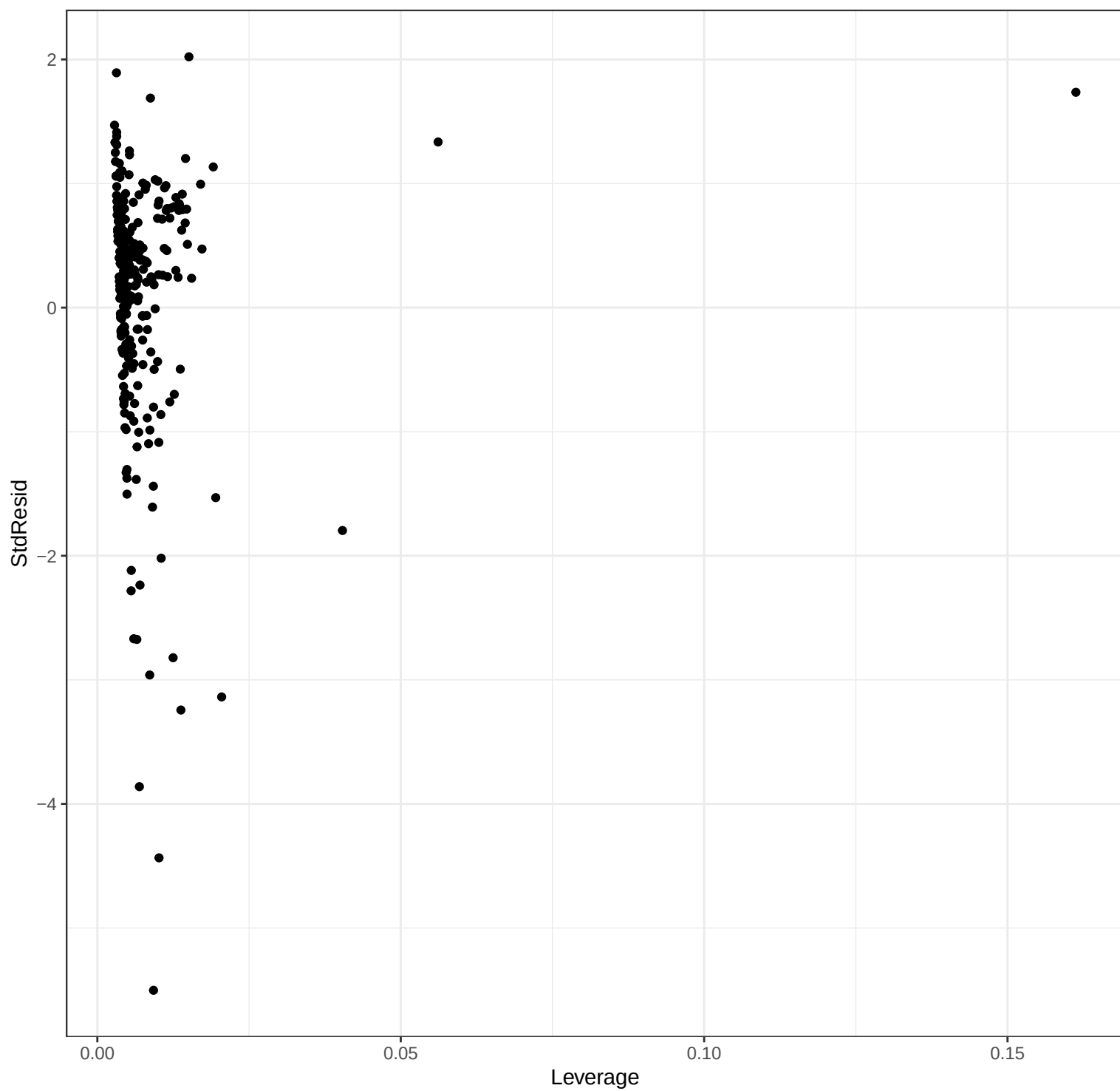
Sr OLS_weighted – Leverage Plot
