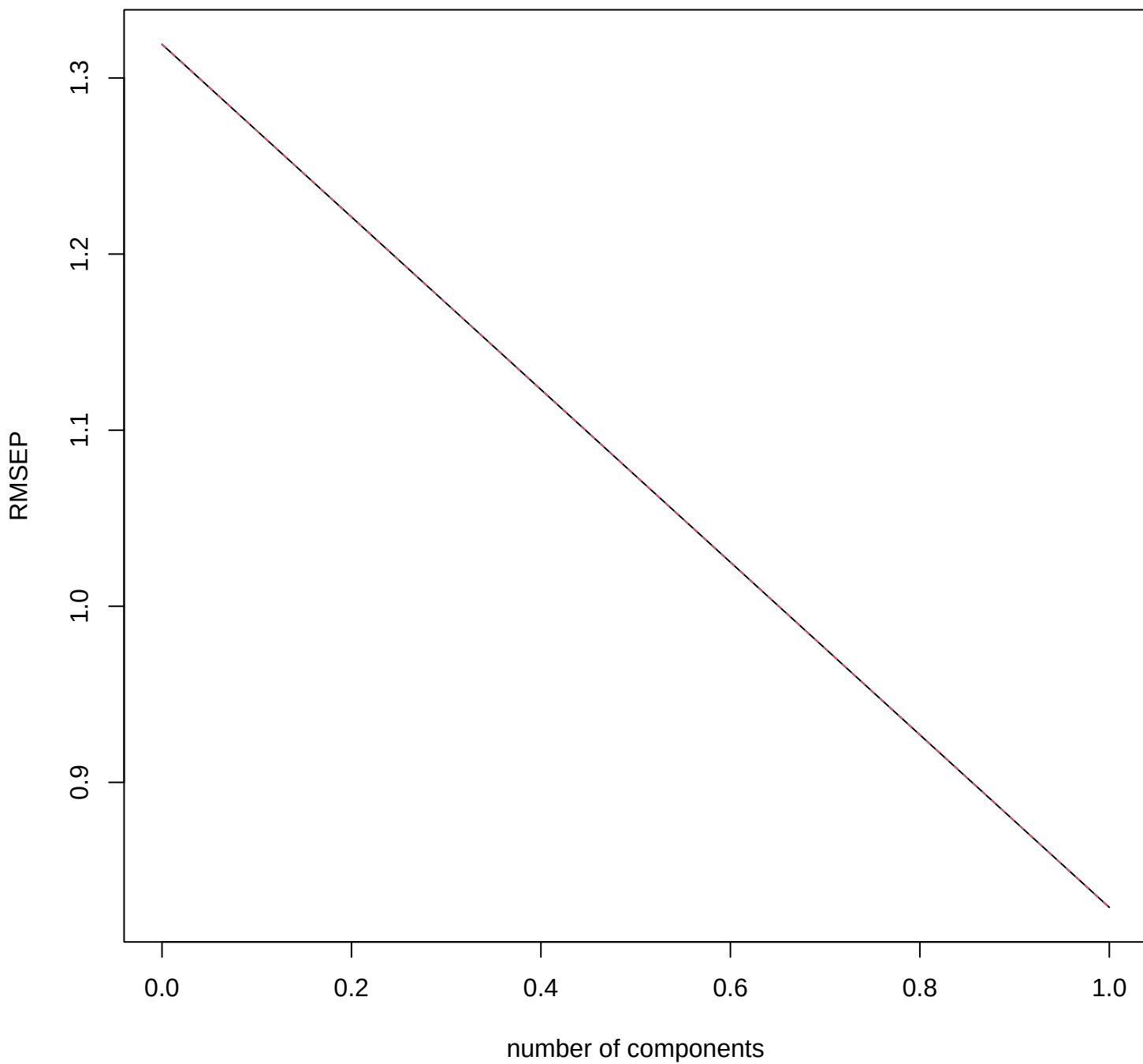
Zr PLS_LOO – RMSEP vs Components
