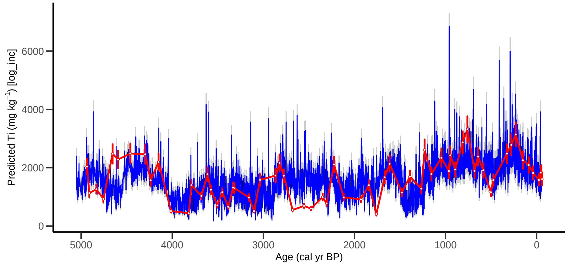
HER42PB: PLSR Ti Predictions with Confidence Interval (log_inc model)
