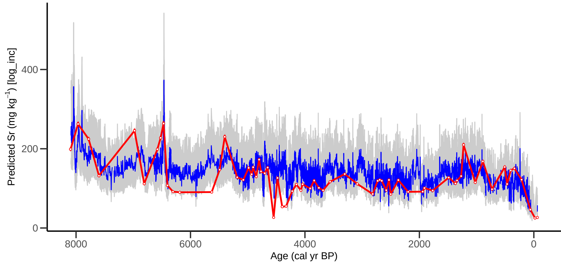
BI10: PLSR Sr Predictions with Confidence Interval (log_inc model)
