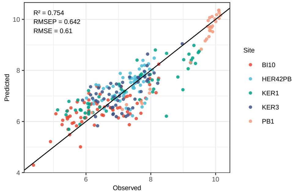
Ti PLS_LOO – Predicted vs Observed (log-space)
