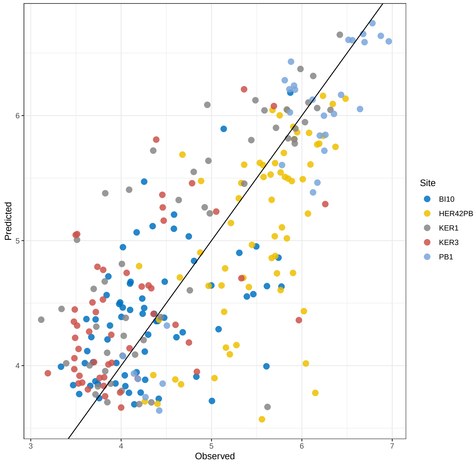
Mn RF – Predicted vs Observed
