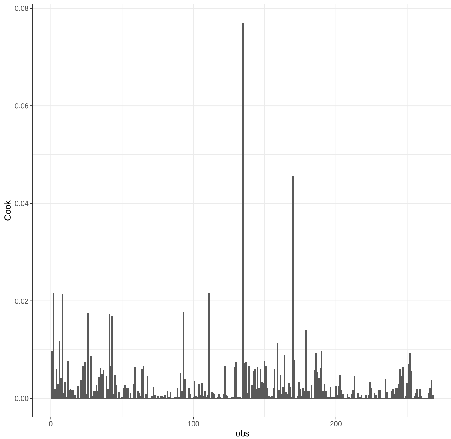
Ti OLS – Cook's Distance
