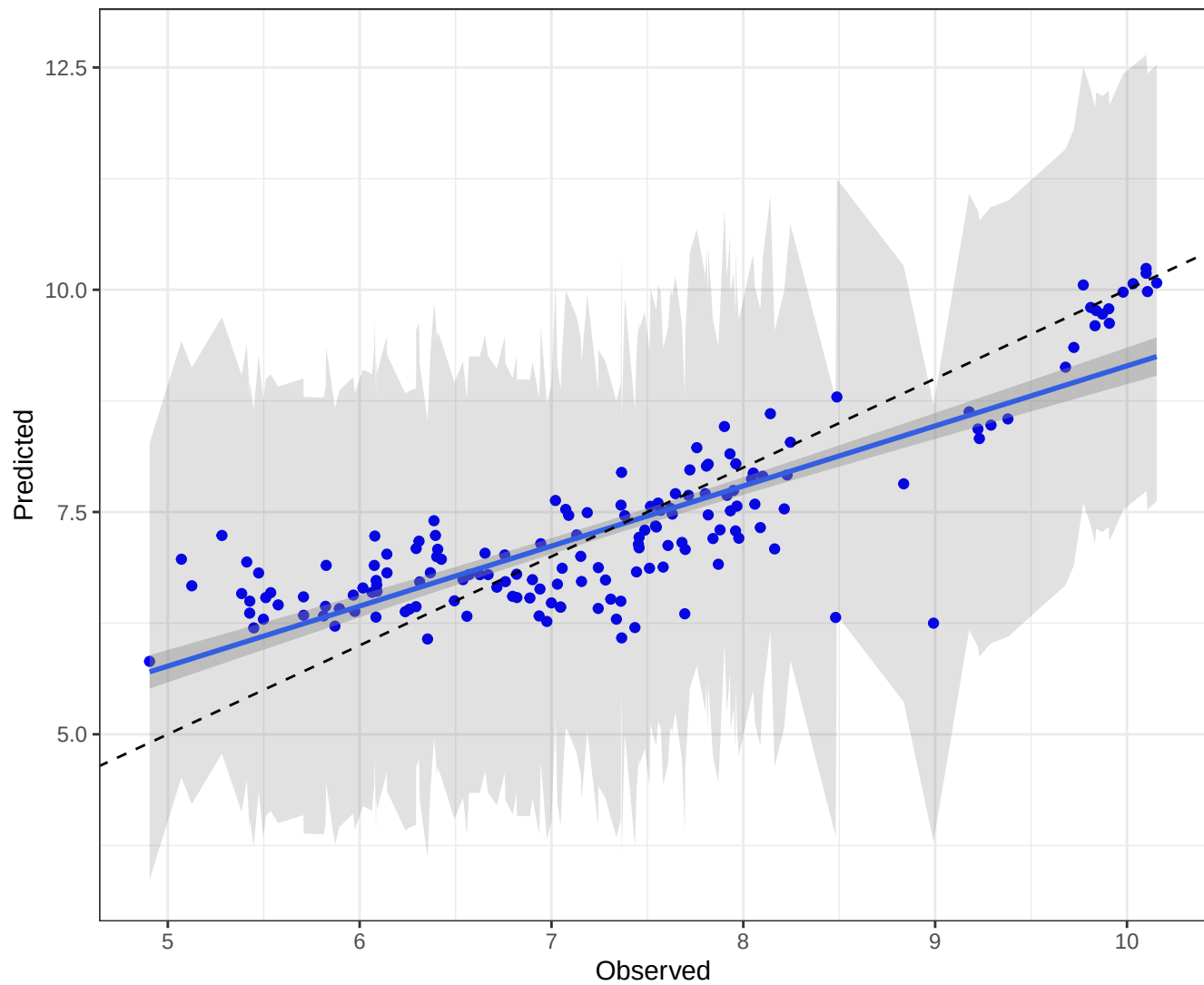
Ti Training: Observed vs Predicted
