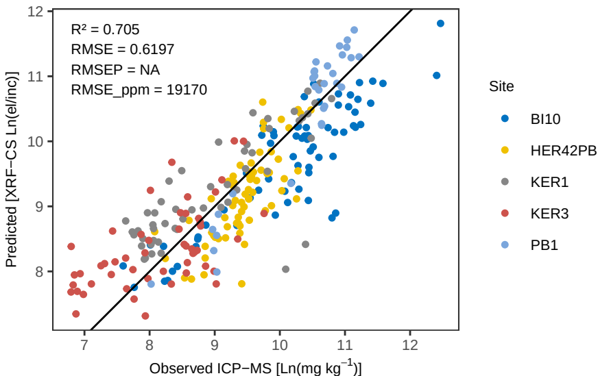
Fe OLS_weighted - Pred vs Obs Training
