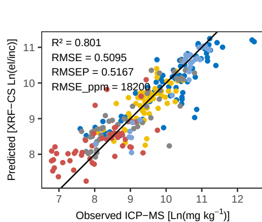
Fe RF – Pred vs Obs Training
