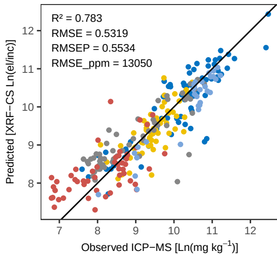
Fe PLS_kfold – Pred vs Obs Training
