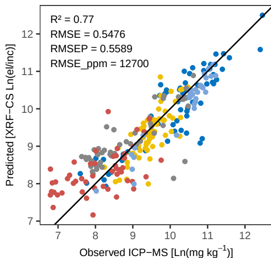
Fe PLS_kfold – Pred vs Obs Training
