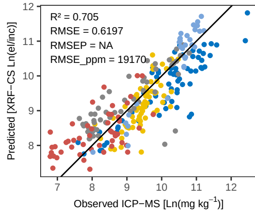
Fe WLS_weighted – Pred vs Obs Training
