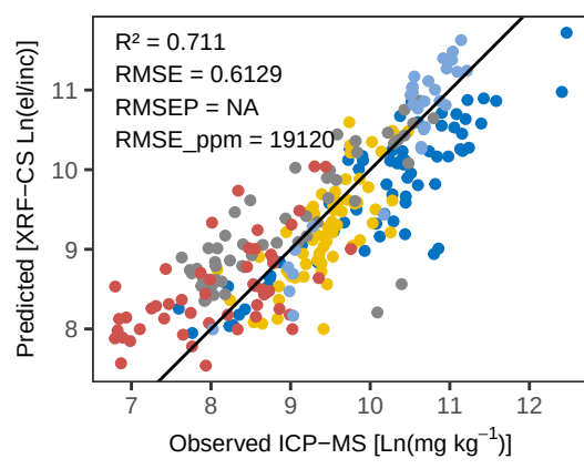
Fe RF – Pred vs Obs Training
