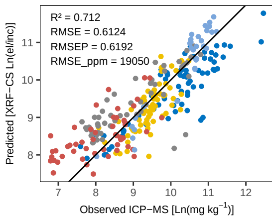
Fe WLS – Pred vs Obs Training
