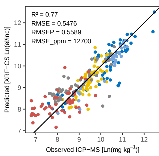
Fe PLS_LOO – Pred vs Obs Training
