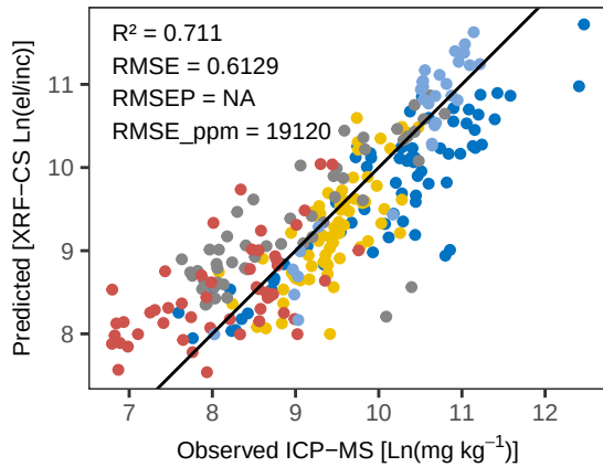
Fe Bayes – Pred vs Obs Training
