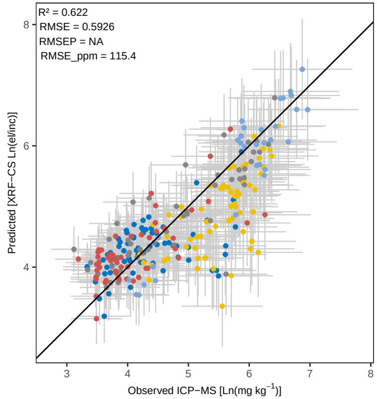
Mn OLS_weighted – Predicted vs Observed (
