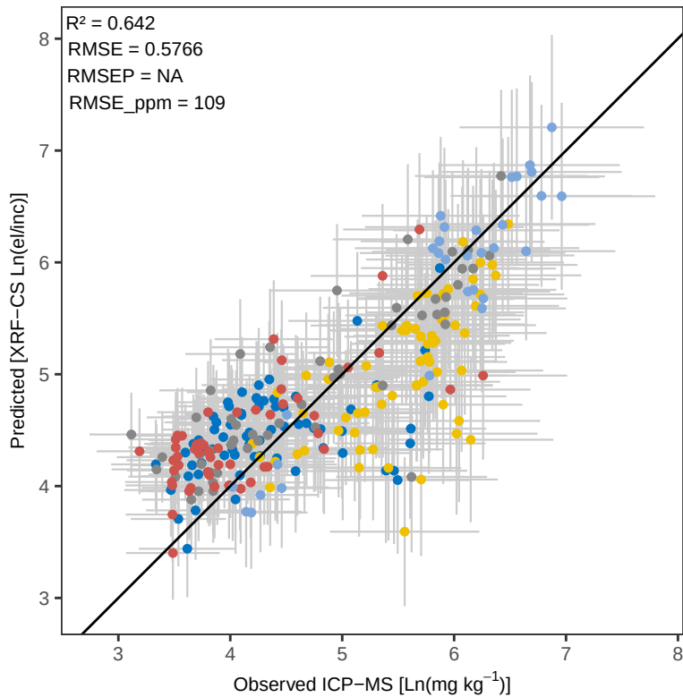
Mn WLS – Predicted vs Observed (
