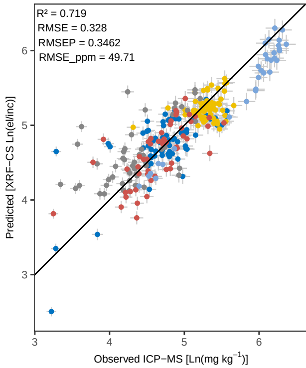
Sr Bayes – Predicted vs Observed (
