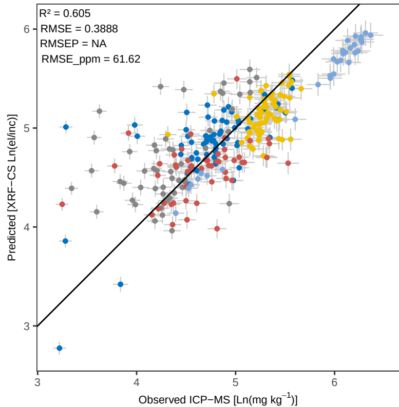
Sr WLS_weighted – Predicted vs Observed (
