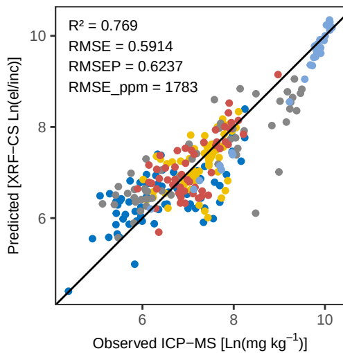
Ti PLS_kfold – Pred vs Obs Training
