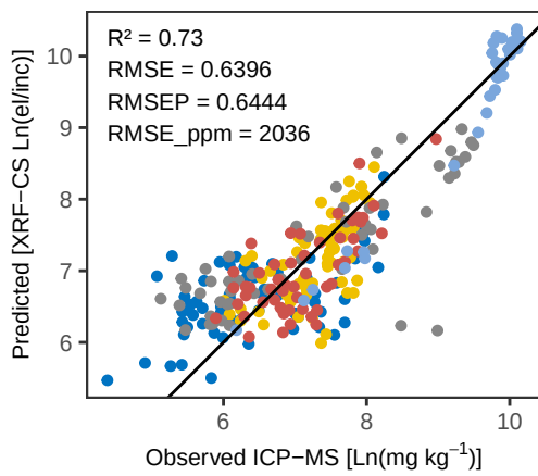
Ti WLS – Pred vs Obs Training
