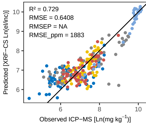
Ti Bayes – Pred vs Obs Training
