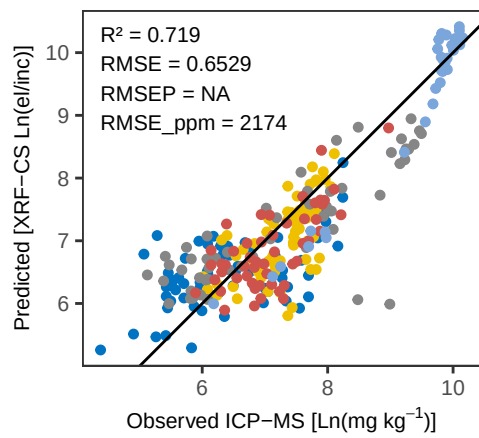
Ti WLS_weighted – Pred vs Obs Training
