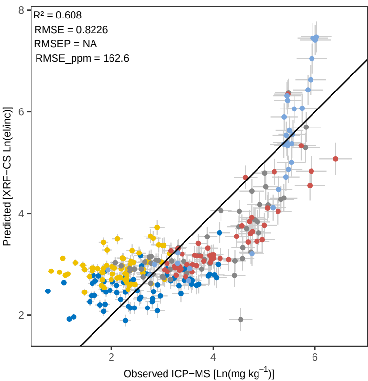
Zr WLS_weighted – Predicted vs Observed (
