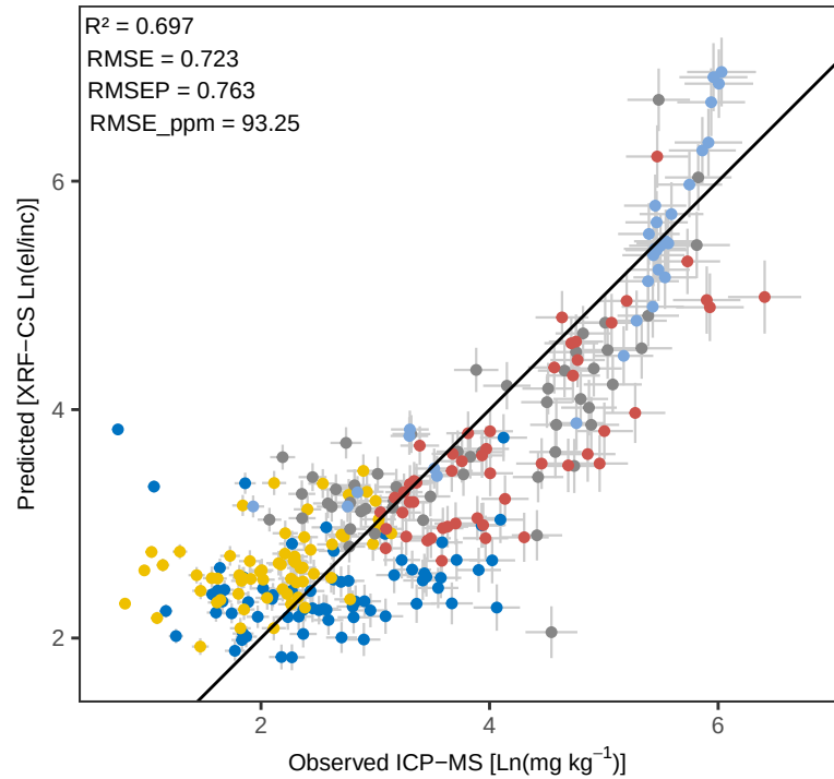
Zr PLS_LOO – Predicted vs Observed (
