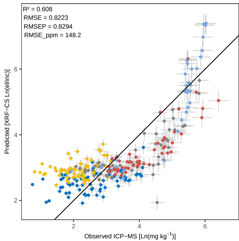
Zr OLS – Predicted vs Observed (
