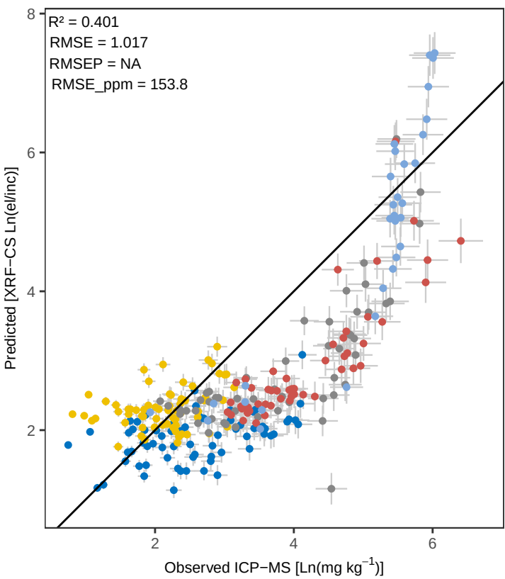
Zr OLS_weighted – Predicted vs Observed (
