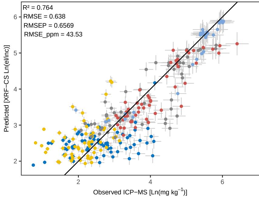
Zr RF – Predicted vs Observed (
