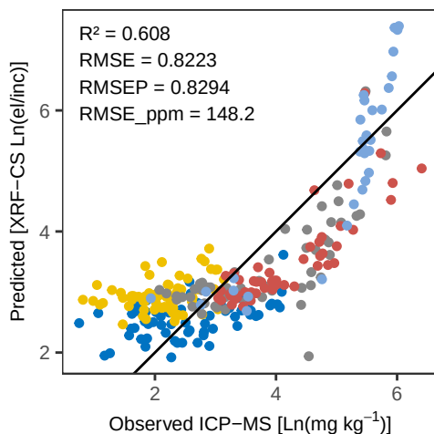
Zr WLS – Pred vs Obs Training
