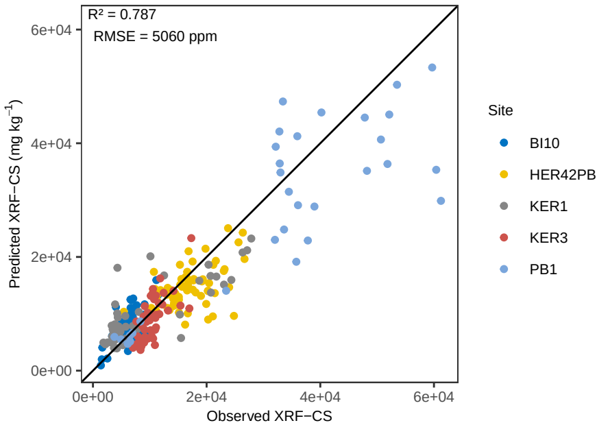
Ca PLS_LOO – Pred vs Obs (Prediction)
