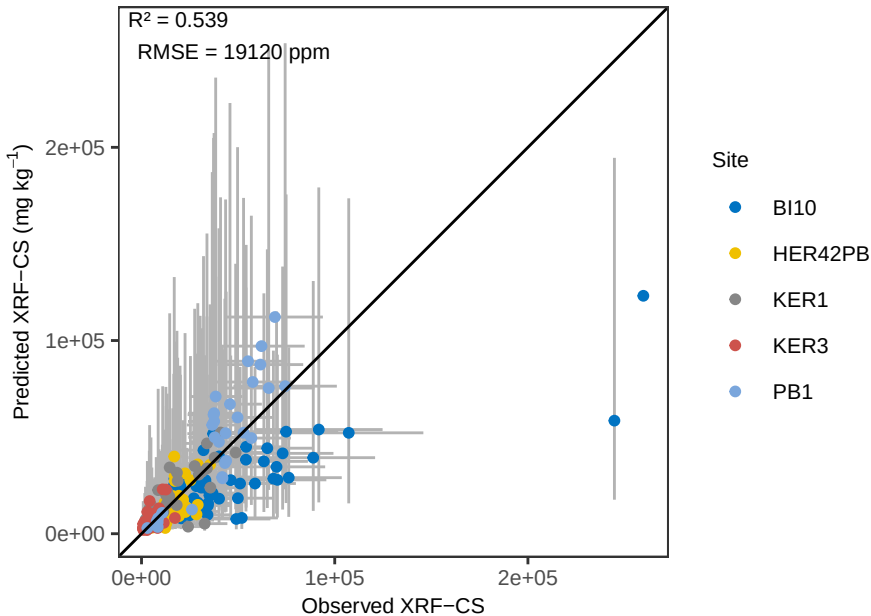
Fe WLS – Pred vs Obs (Prediction)
