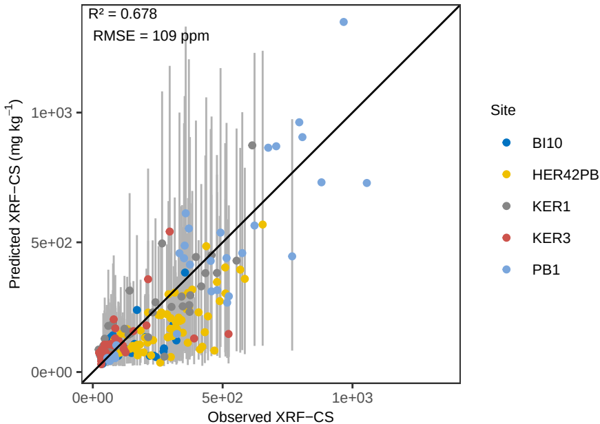
Mn WLS – Pred vs Obs (Prediction)
