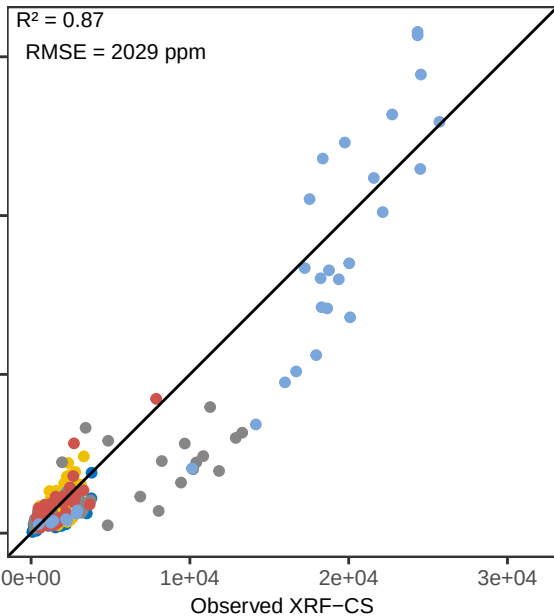
Ti PLS_LOO – Pred vs Obs (Prediction)
