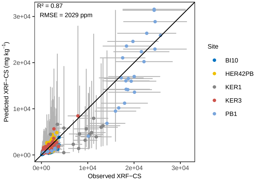
Ti PLS_kfold - Pred vs Obs (Prediction)
