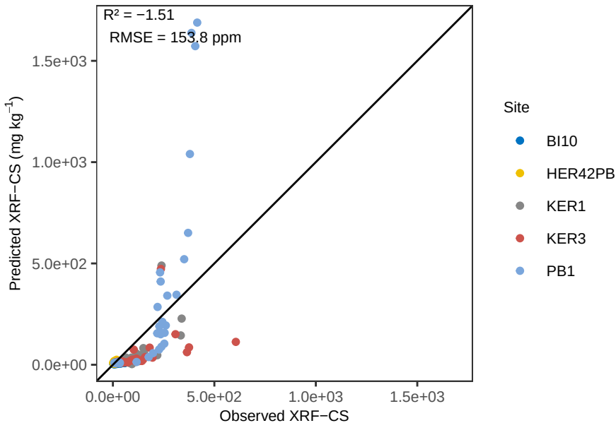
Zr OLS_weighted – Pred vs Obs (Prediction)
