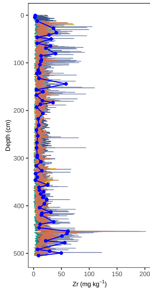
Site BI10 – Zr (depth, all models)
