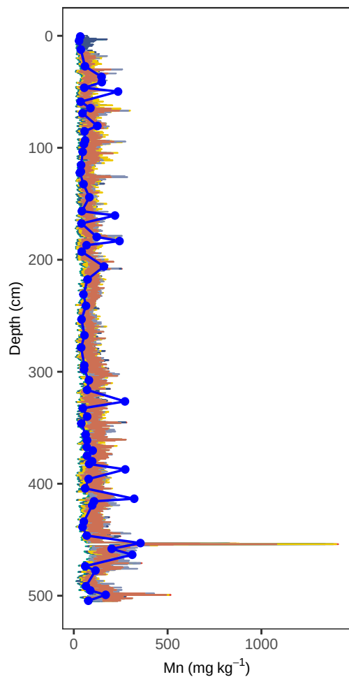
Site BI10 – Mn (depth, all models)
