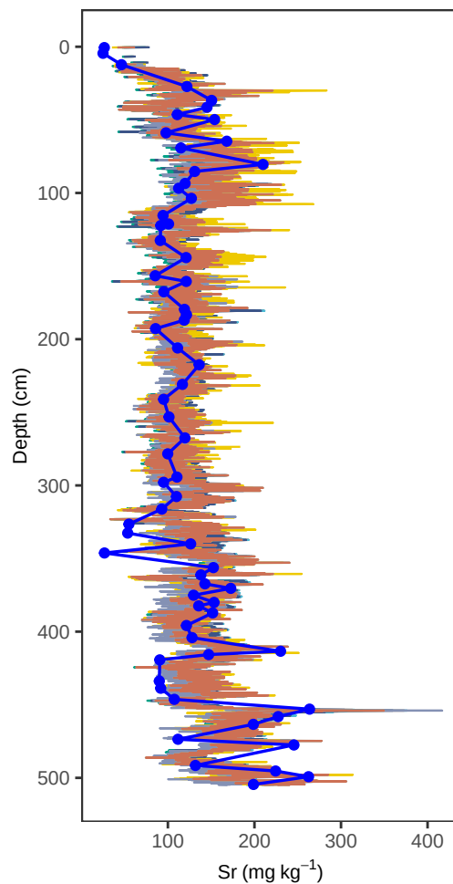
Site BI10 – Sr (depth, all models)
