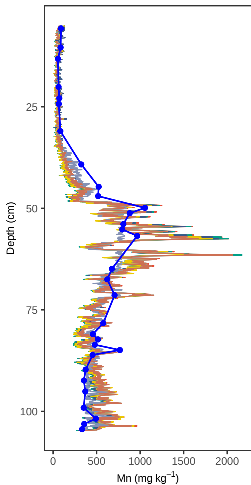
Site PB1 – Mn (depth, all models)
