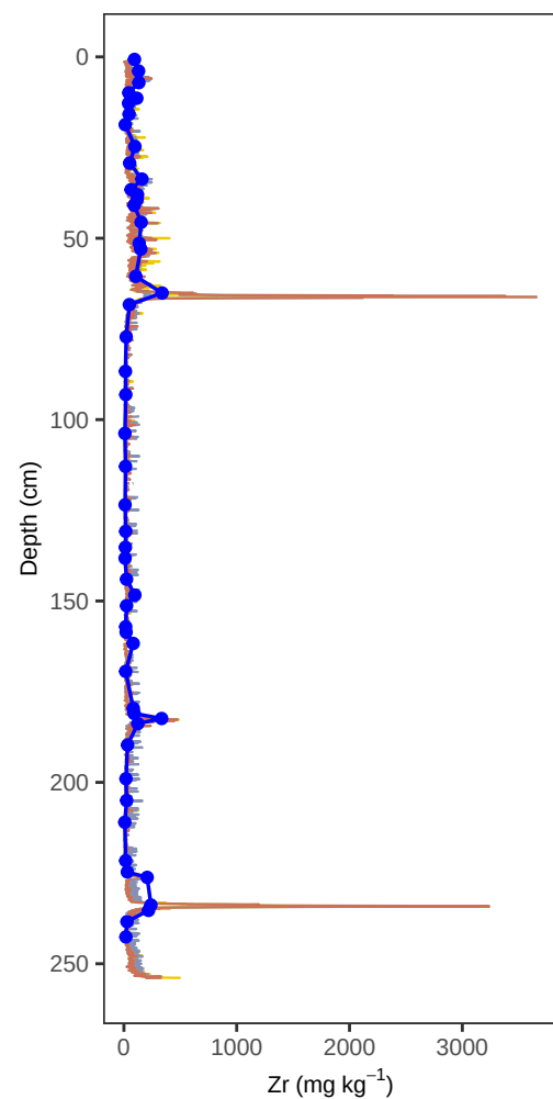
Site KER1 – Zr (depth, multivariate)
