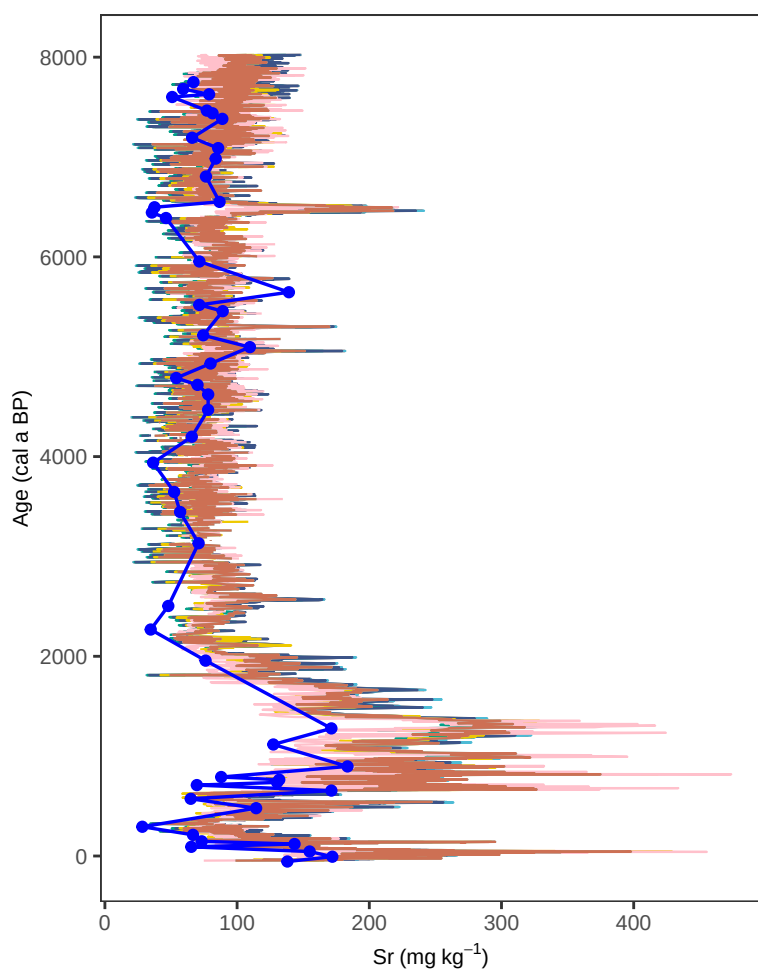
Site KER1 – Sr (age, all models)
