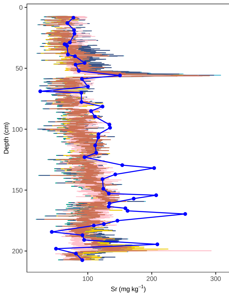
Site KER3 – Sr (depth, all models)
