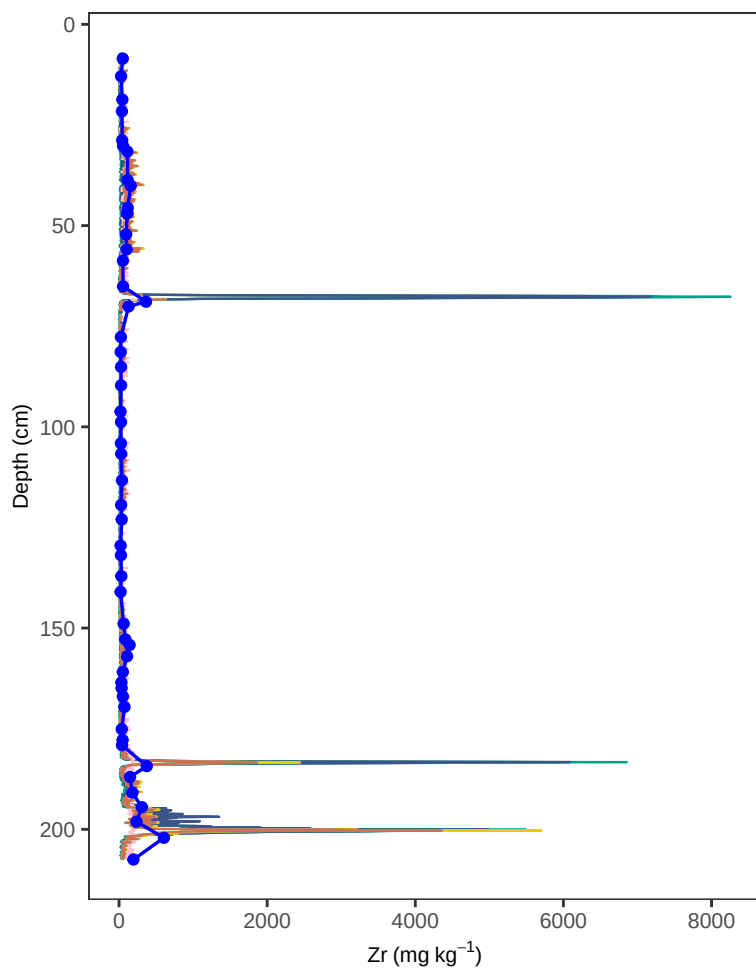
Site KER3 – Zr (depth, all models)
