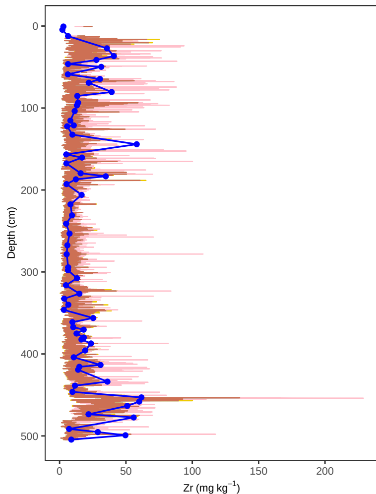
Site BI10 – Zr (depth, multivariate)
