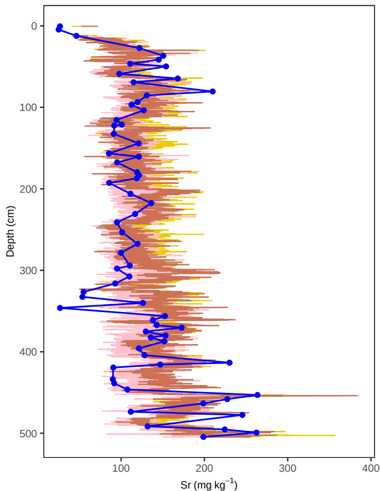
Site BI10 – Sr (depth, multivariate)
