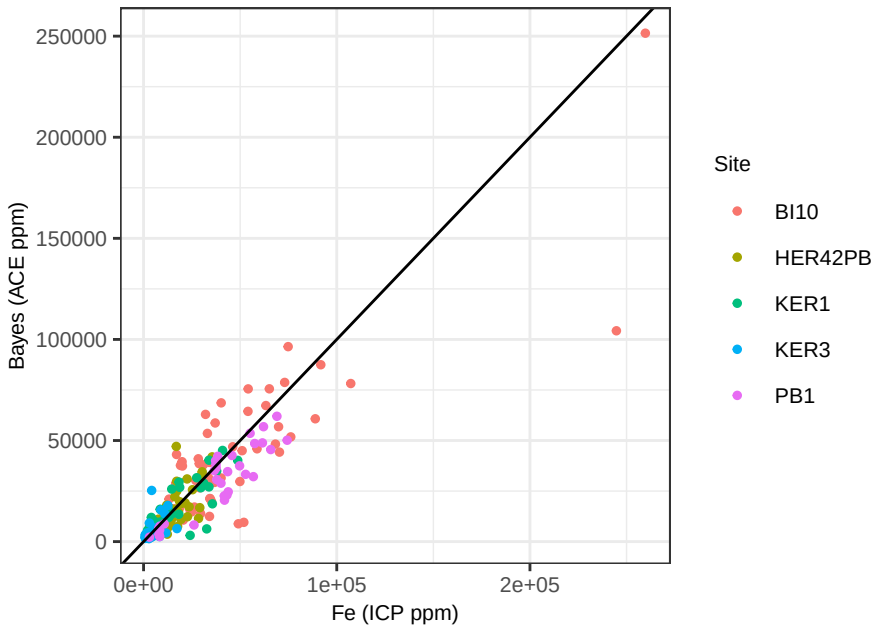
Fe Bayes – ACE Pred vs Obs
