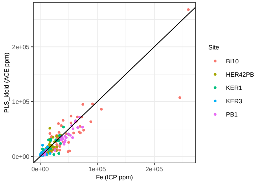
Fe PLS_kfold - ACE Pred vs Obs
