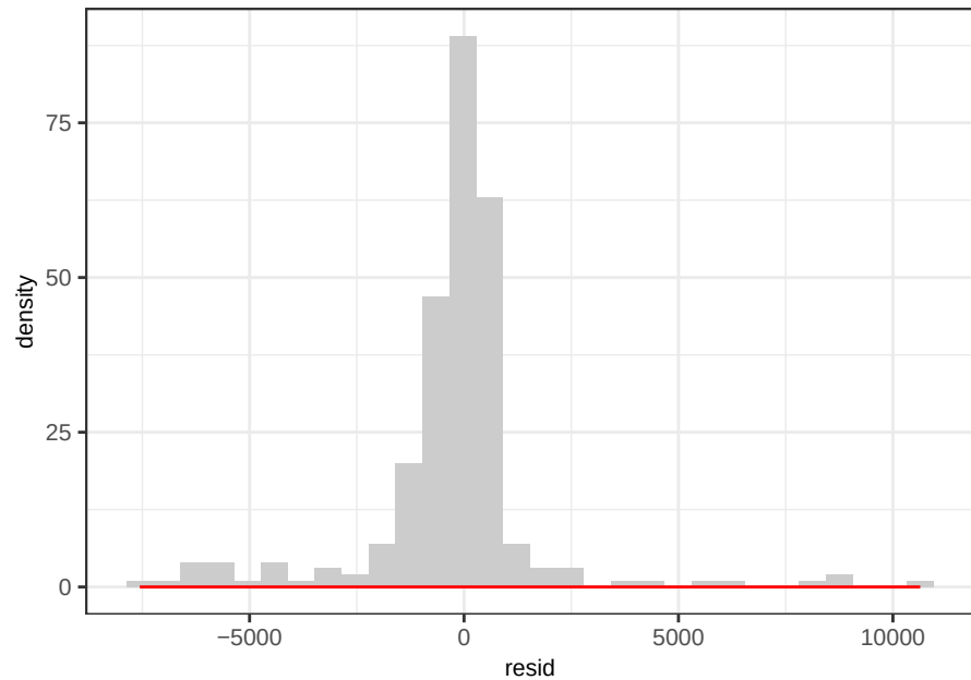
Ti OLS – ACE Residuals
