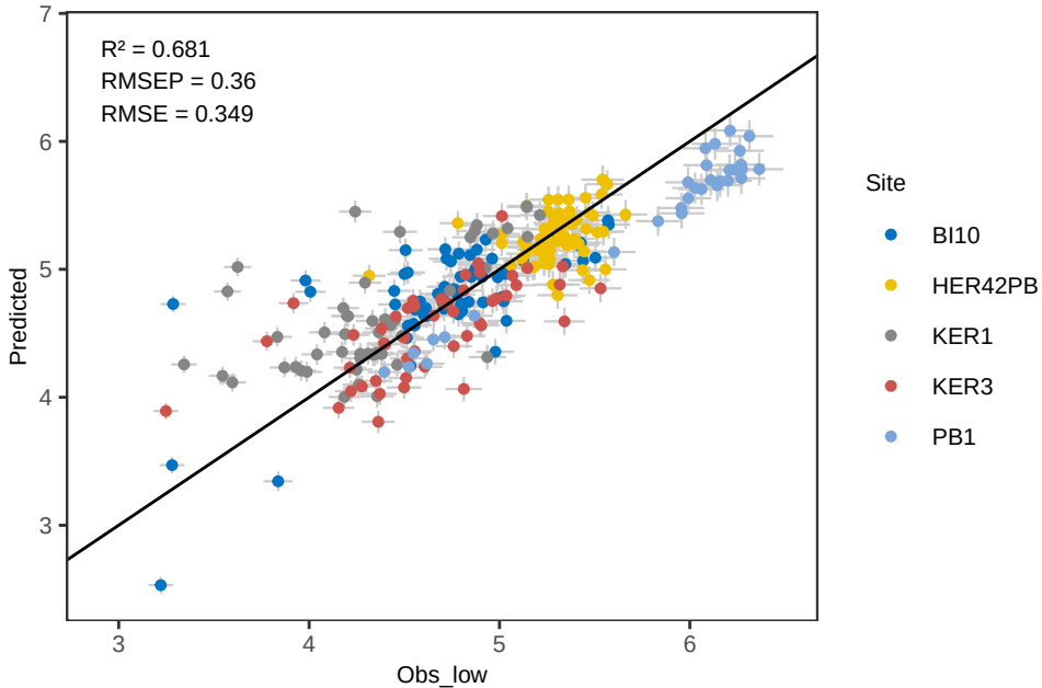
Sr PLS_kfold - Predicted vs Observed
