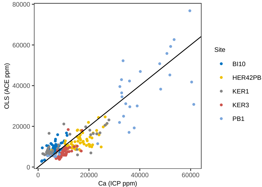
Ca OLS – ACE Pred vs Obs
