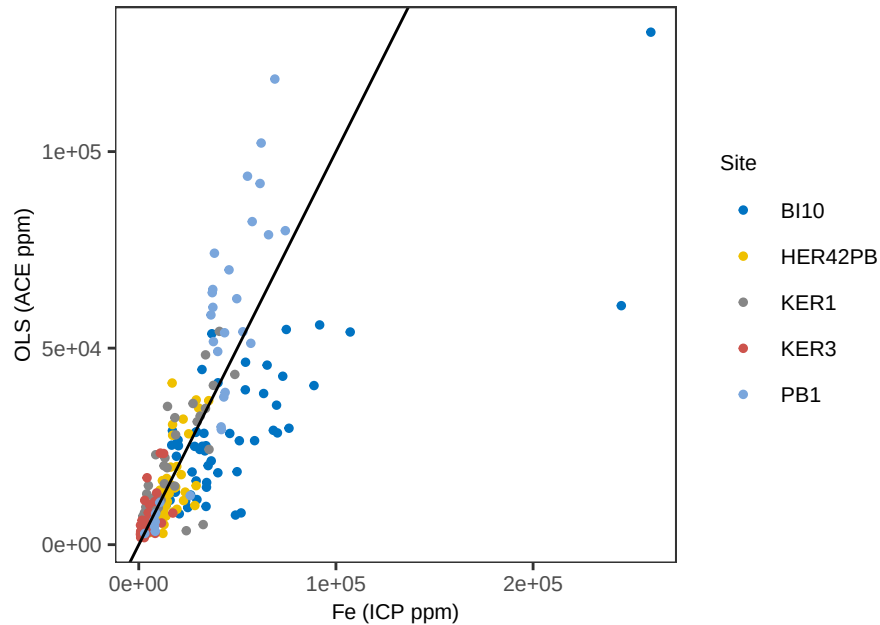
Fe OLS – ACE Pred vs Obs
