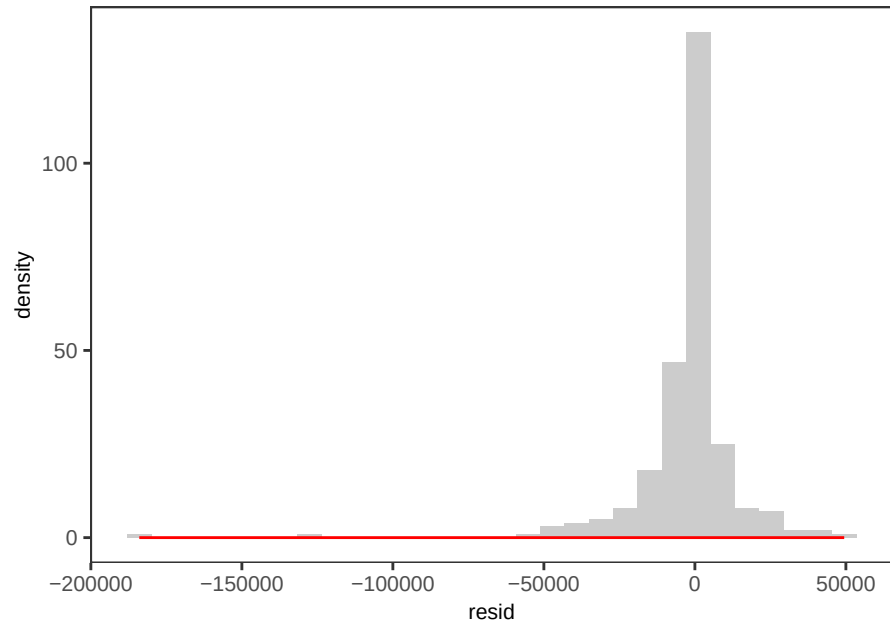
Fe OLS - ACE Residuals
