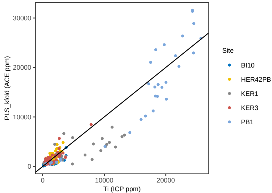
Ti PLS_kfold - ACE Pred vs Obs
