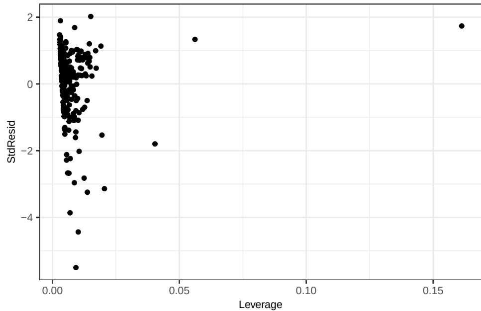
Sr OLS_weighted – Leverage
