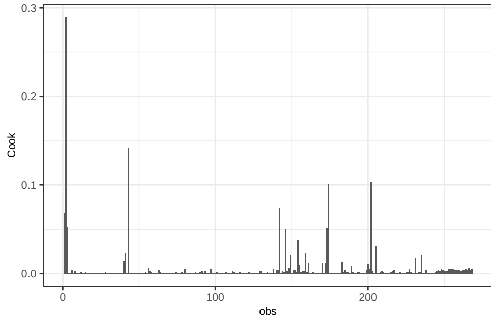
Sr OLS_weighted – Cook's Distance
