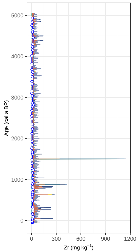
Site HER42PB – Zr (age, all models)
