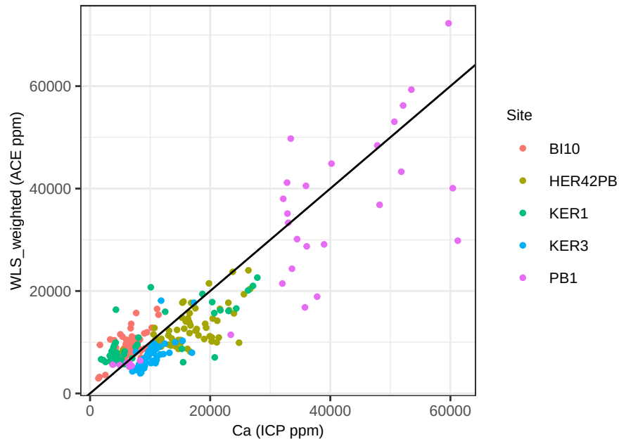
Ca WLS_weighted – ACE Pred vs Obs
