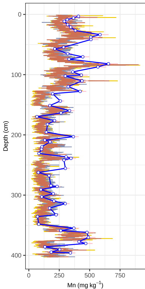
Site HER42PB – Mn (depth, multivariate)
