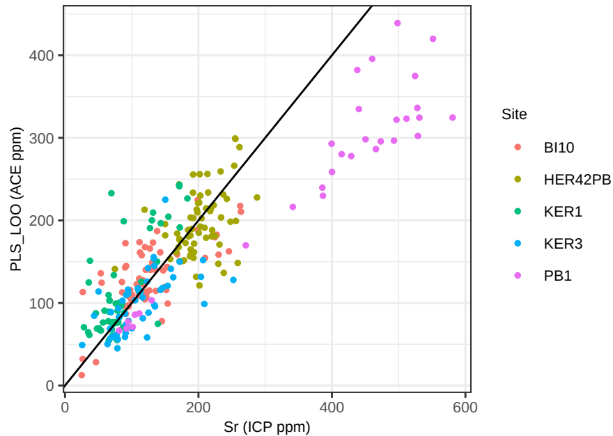
Sr PLS_LOO – ACE Pred vs Obs
