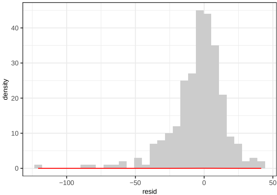
Sr RF – ACE Residuals
