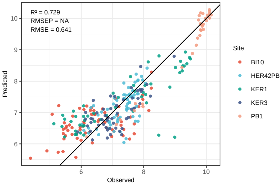
Ti WLS – Predicted vs Observed
