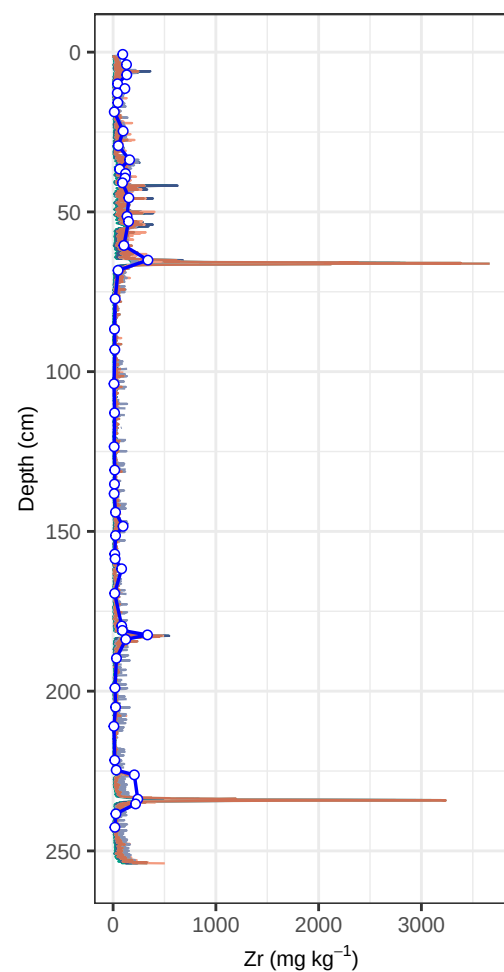
Site KER1 – Zr (depth, all models)
