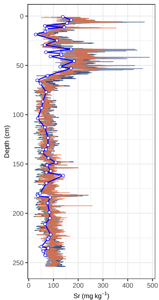
Site KER1 – Sr (depth, all models)
