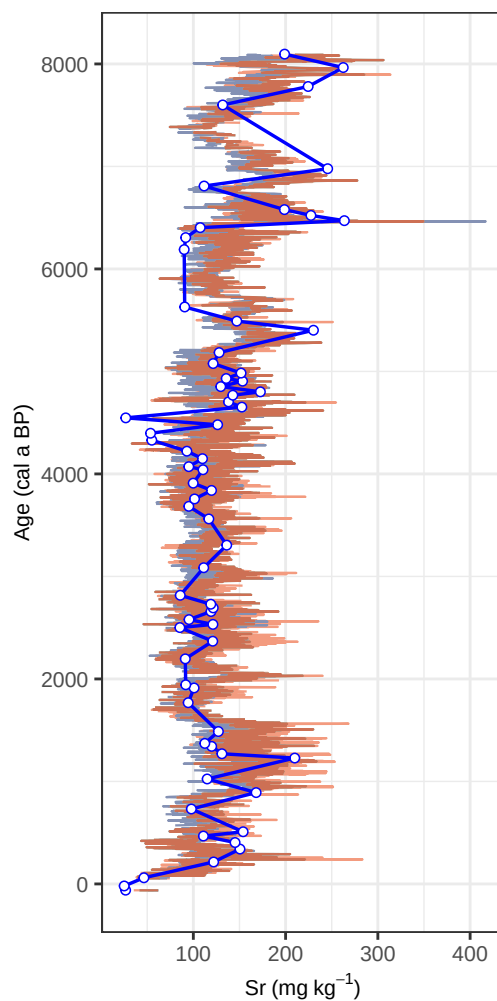
Site BI10 – Sr (age, multivariate)
