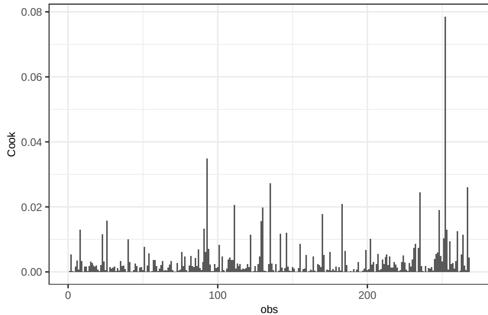
Mn WLS – Cook's Distance
