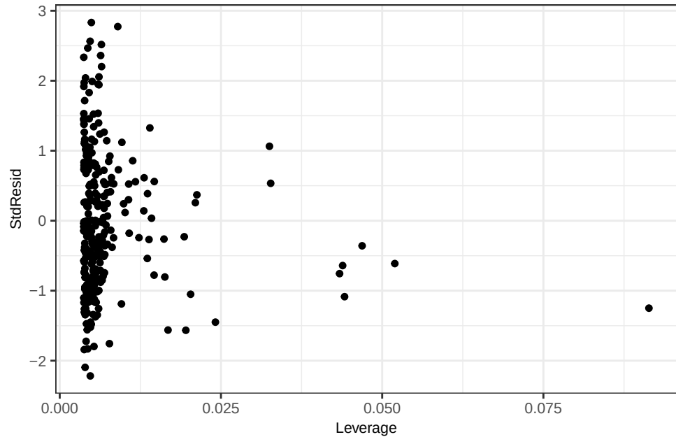
Mn WLS – Leverage
